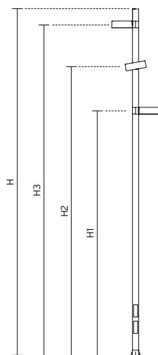
PLIZAR TOWER 310 with MIZAR luminaires
